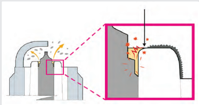
Secondary Micro-Discharge & Self-Cleaning Action of the Iridium IX
