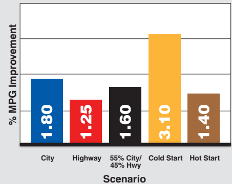
AMSOIL SAE 5W-40 Fuel Economy Results – FTP Cycle
